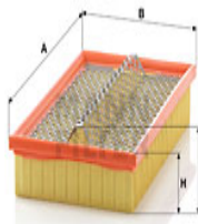
Air Filters C 2256 EM-30061
